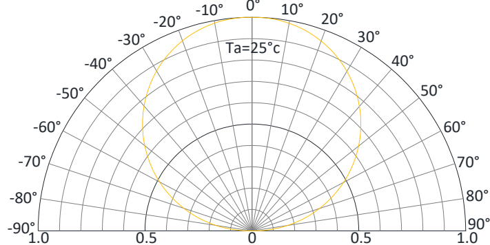
Radiation Pattern
