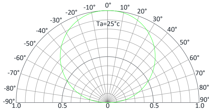
Radiation Pattern
