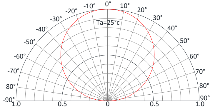
Radiation Pattern
