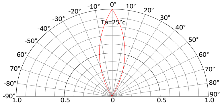
Radiation Pattern
