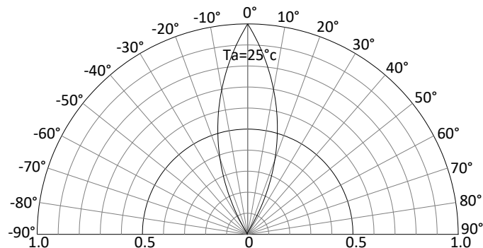
Radiation Pattern
