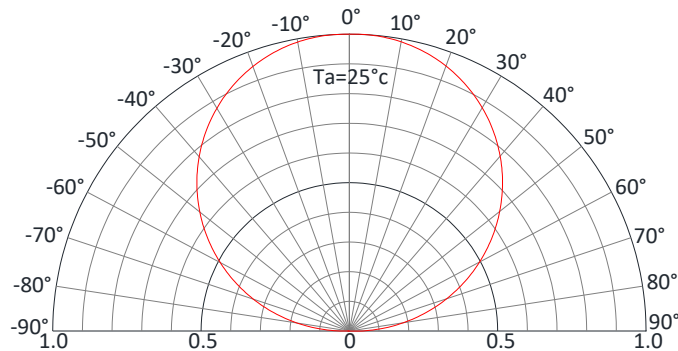
Radiation Pattern
