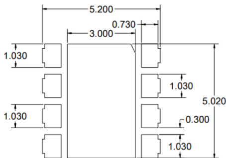
PCB pad design recommendations
