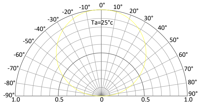
Radiation Pattern
