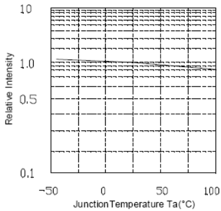
Figure 5: Relative Luminous Flux vs. Temperature
