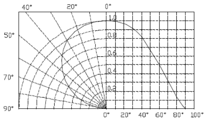
Figure 6: Radiation Pattern
