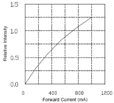
Figure 4:Relative Luminous Flux vs. Forward Current
