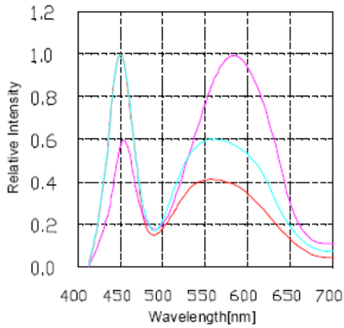
Figure 1:Wavelength Characteristics
