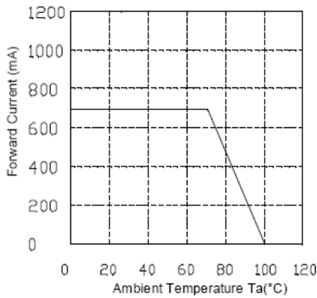
Figure 3:Forward Current vs. Temperature
