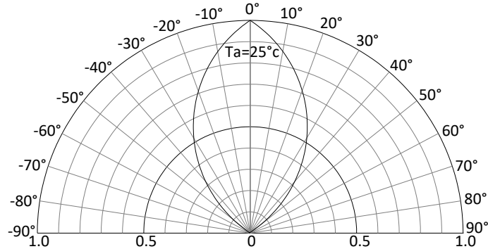
Radiation Pattern
